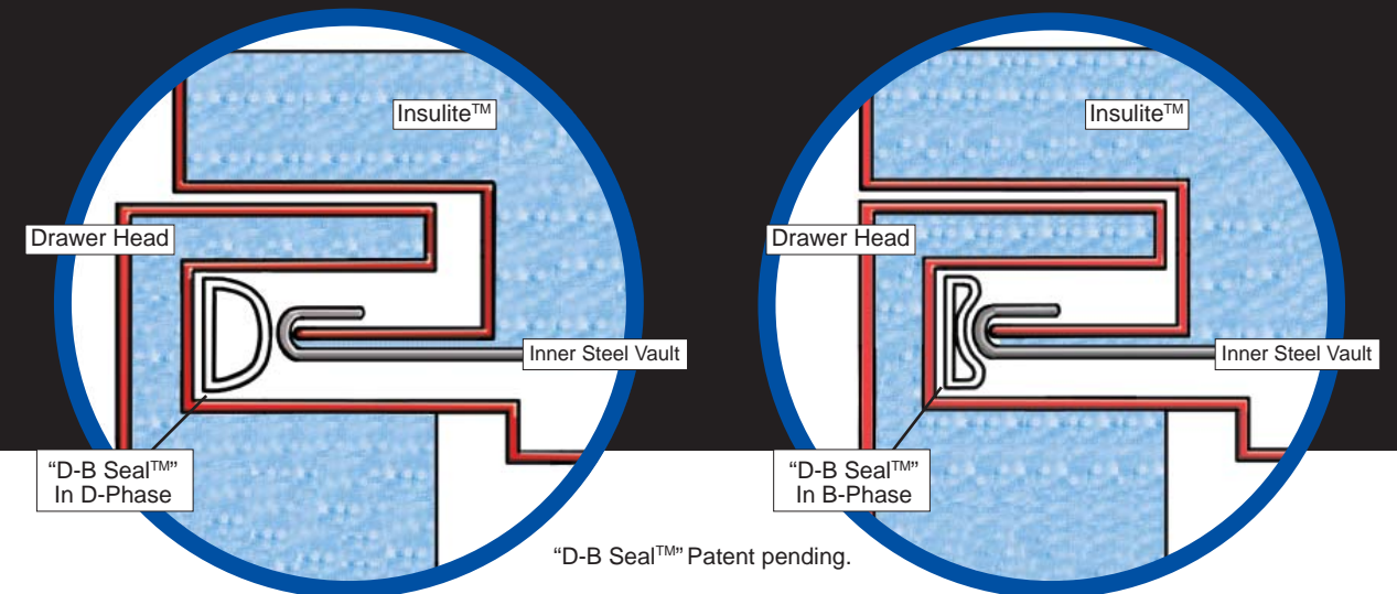
Cross-section of drawer head joint in open position with D-B Seal™ in "D-Phase"
